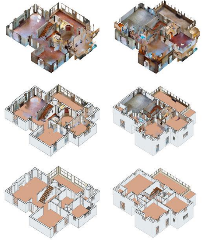
Apartment - Point Cloud to Revit
